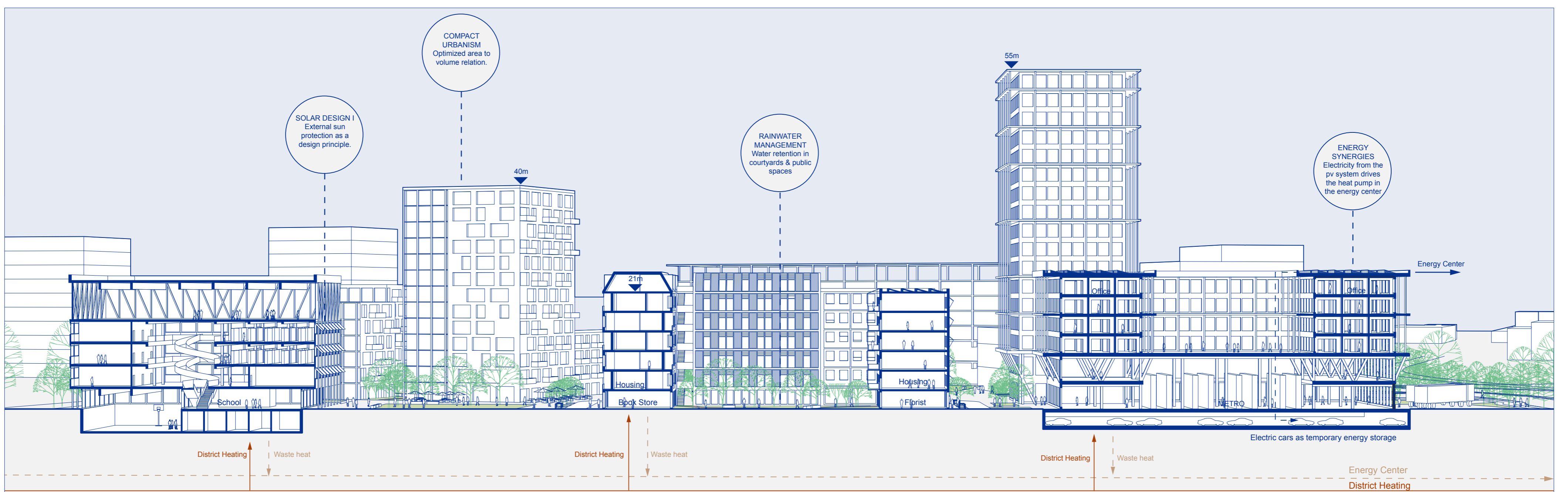
Section 1:500
