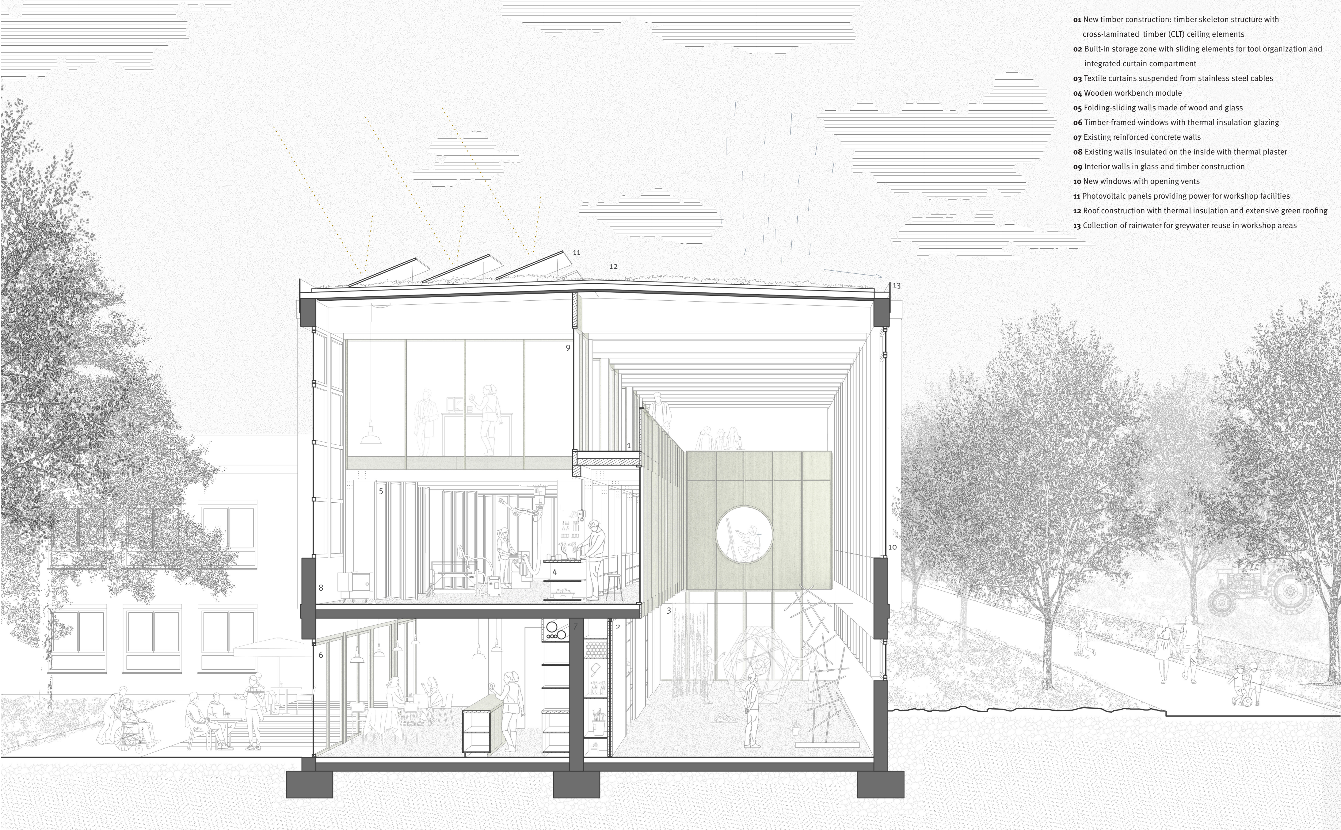
Cross section - hall, workshop, cafe M 1:50
