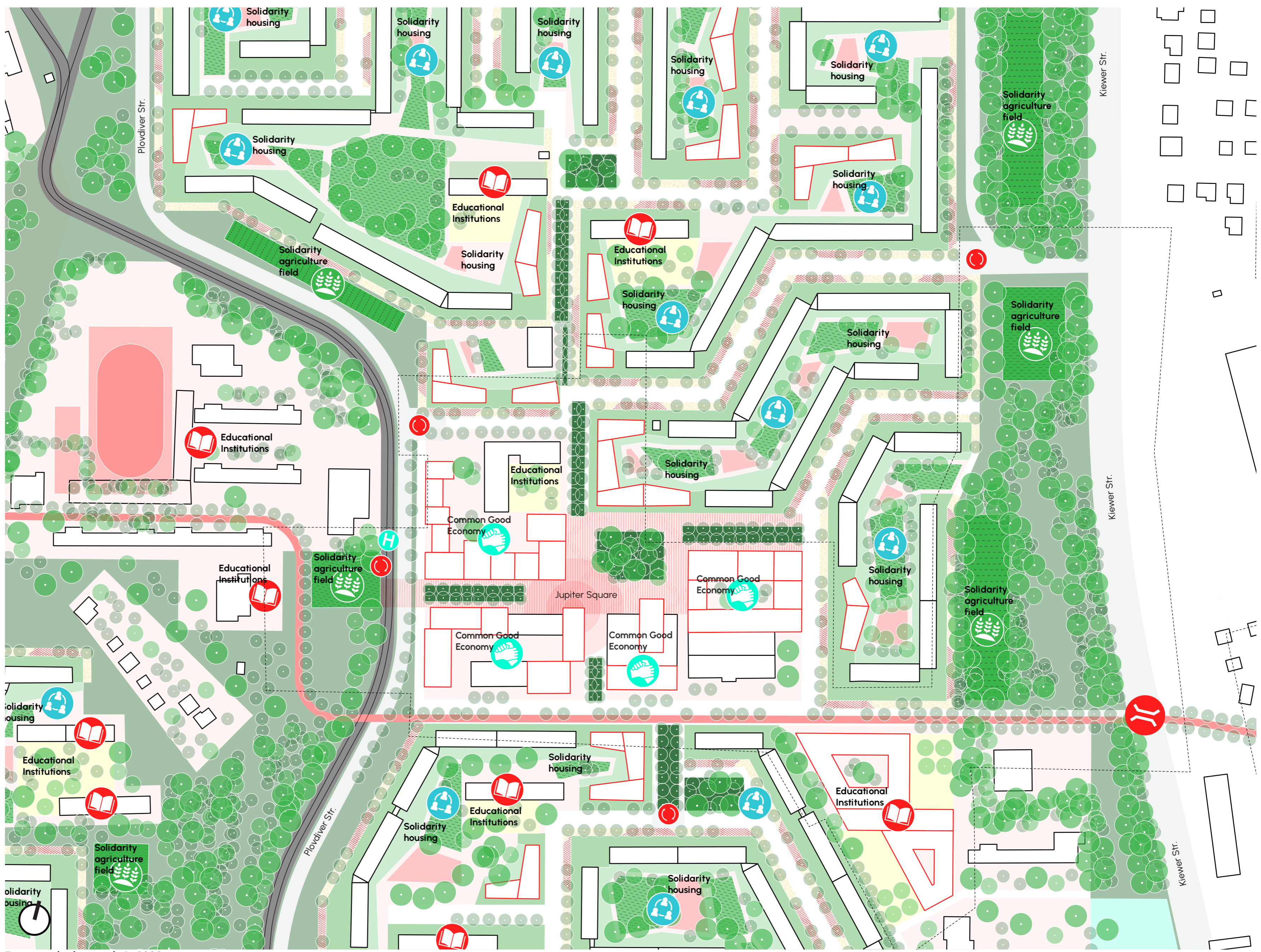
Framework plan, scale 1 : 2000
